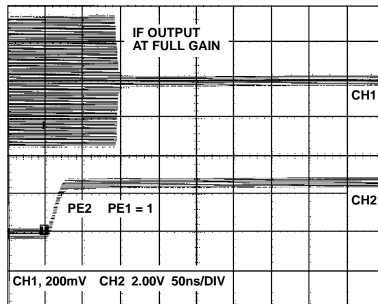
FIGURE 48. TX TO RX IF OUTPUT SWITCHING TIME
