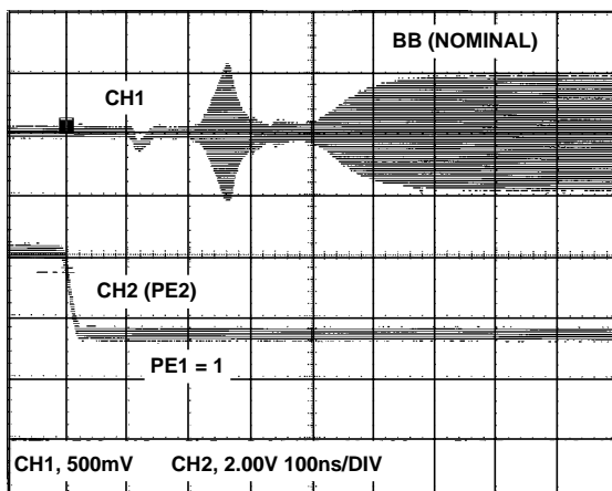
FIGURE 25. TX TO RX BASEBAND SWITCHING TIME
