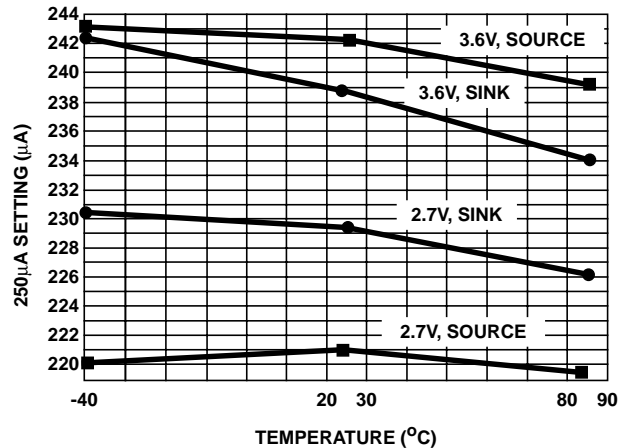
FIGURE 12. CHARGE PUMP 250µA SETTING SINK AND SOURCE CURRENT OVER TEMPERATURE AND VOLTAGE
