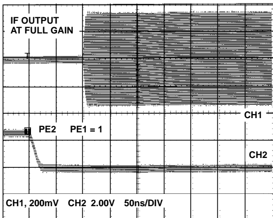
FIGURE 47. RX TO TX IF OUTPUT SWITCHING TIME
