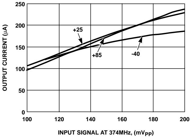
FIGURE 30. TYPICAL IF DETECTOR OUTPUT CURRENT AT ALL V_{CC}
