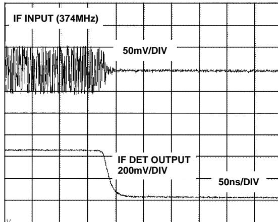
FIGURE 32. IF DETECTOR RESPONSE, FALL TIME
