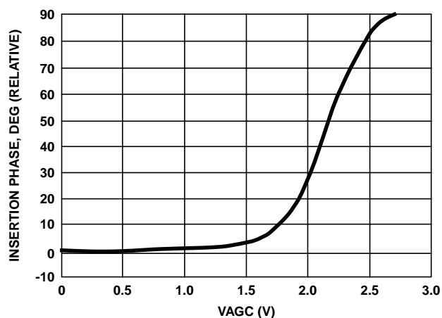
FIGURE 44. TX INSERTION PHASE vs VAGC
