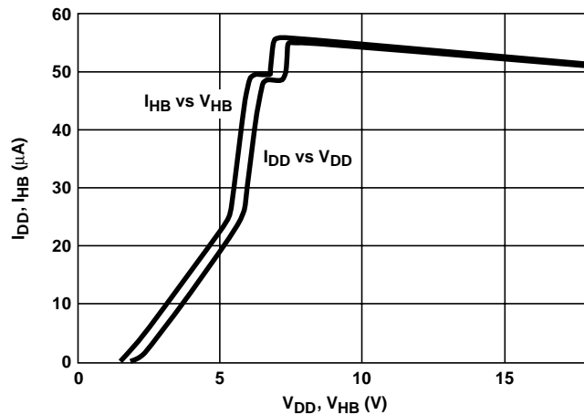
FIGURE 15. BIAS CURRENT vs VOLTAGE
