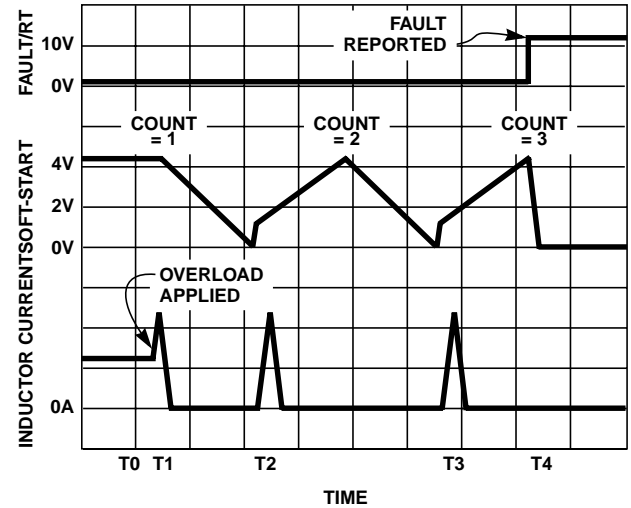
FIGURE 8. OVER-CURRENT OPERATION
