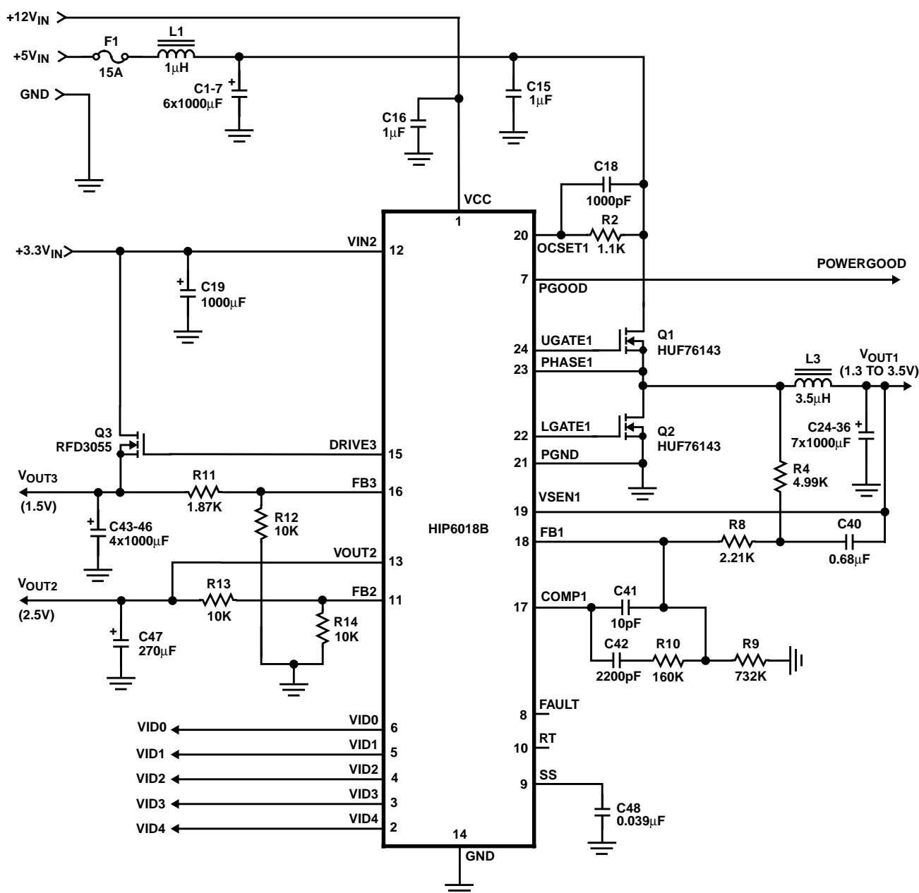
FIGURE 15. APPLICATION CIRCUIT
