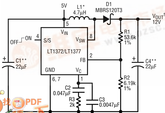
5V-to-12V Boost Converter
