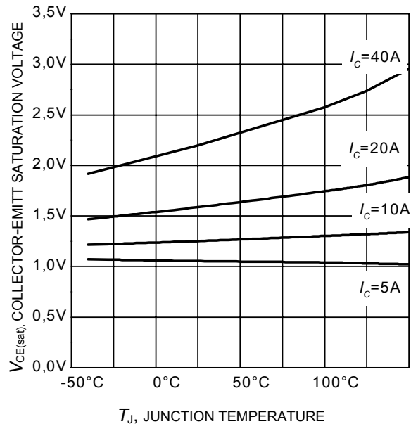
T_j , JUNCTION TEMPERATURE Figure 8. Typical collector-emitter saturation voltage as a function of junction temperature ( V_{GE} = 15\text{V} )
