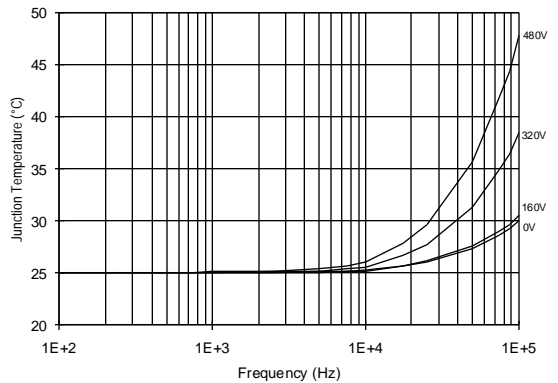
Figure 8. IR2131 T J vs. Frequency (IRF830) R GATE = 20Ω, V CC = 15V
