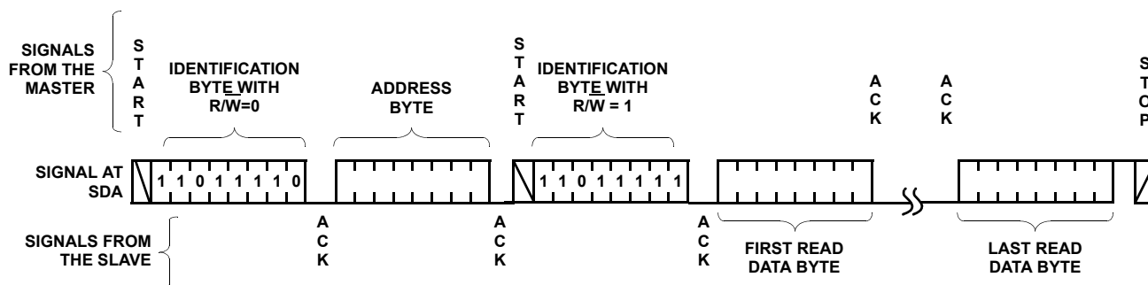
FIGURE 16. READ SEQUENCE
