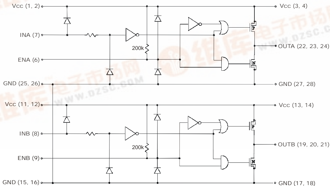
Figure 1 - Functional Diagram
