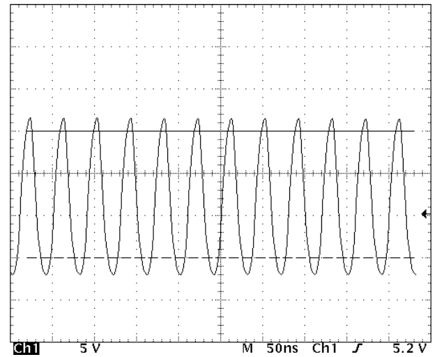
Figure 13 50MHz Burst Repetition Frequency
