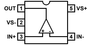
EL5163 (5-PIN SOT-23, SC-70) TOP VIEW
