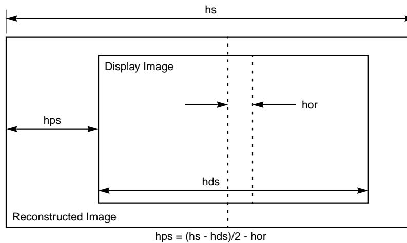
Figure 9.17 Horizontal Pan and Scan Calculation
