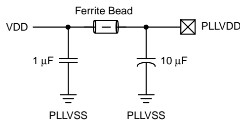
Figure 2.2 PLLVD Decoupling Circuit
