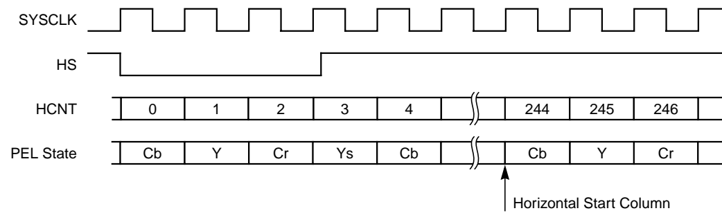
Figure 9.6 Horizontal Input Timing
