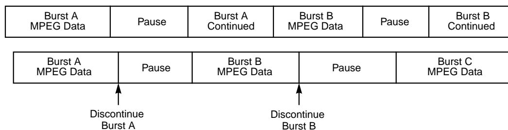
Figure 10.9 Inserting Pause Bursts in the MPEG Formatter Output
