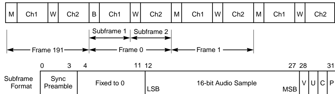
Figure 10.14 IEC958 Syntax
