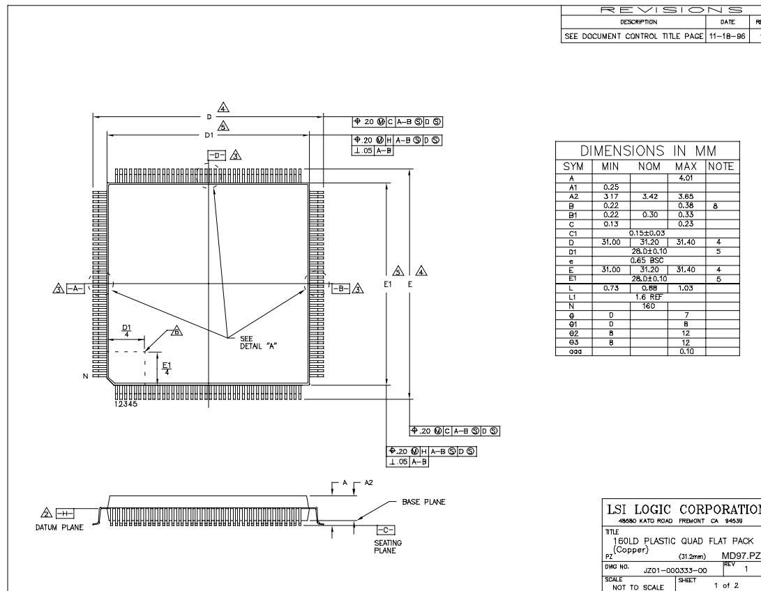
Figure 11.17 160-Pin PQFP (PZ) Mechanical Drawing (Sheet 1 of 2)
