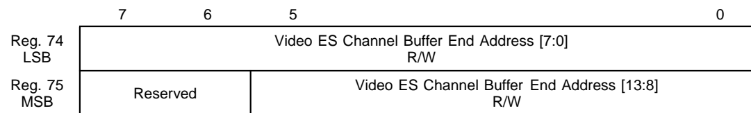
Figure 4.24 Registers 74 and 75 (0x04A and 0x04B) Video ES Channel Buffer End Address [13:0]
