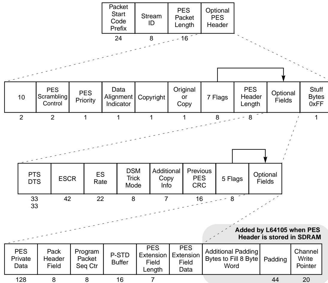
Figure 6.7 PES Packet Structure
