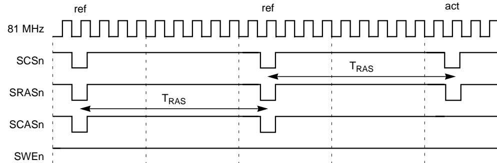
Figure 7.4 SDRAM Timing Requirements for Refresh
