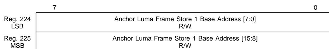
Figure 4.70 Registers 224 and 225 (0x0E0 and 0x0E1) Anchor Luma Frame Store 1 Base Address [15:0]
