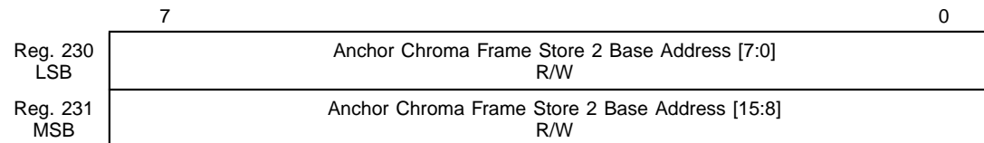
Figure 4.73 Registers 230 and 231 (0x0E6 and 0x0E7) Anchor Chroma Frame Store 2 Base Address [15:0]
