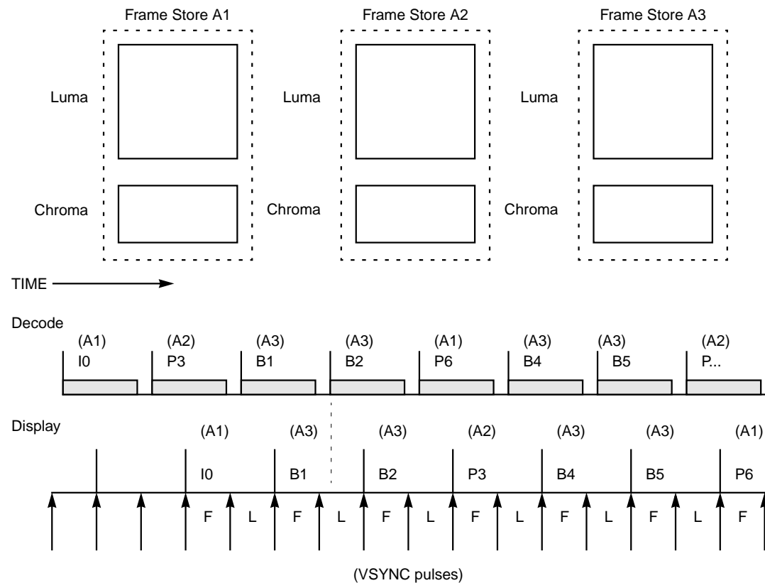
Figure 8.4 Frame Store Organization in Normal Mode
