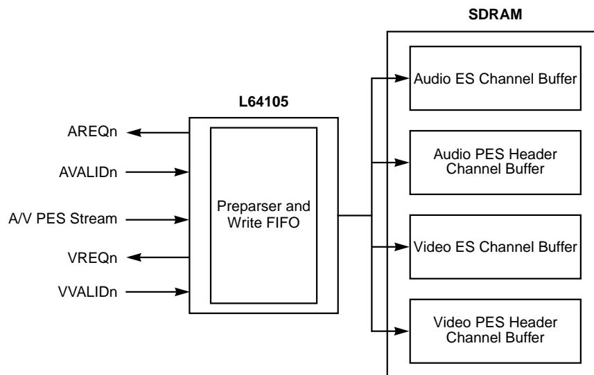
Figure 6.14 Parsing an Audio/Video PES Transport Stream
