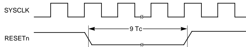
Figure 11.11 Reset Timing
