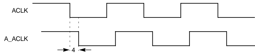
Figure 11.14 A_ACLK Timing
