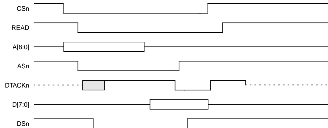
Figure 5.2 Motorola Mode Write Timing
