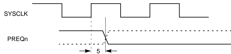
Figure 11.15 PREQn Timing
