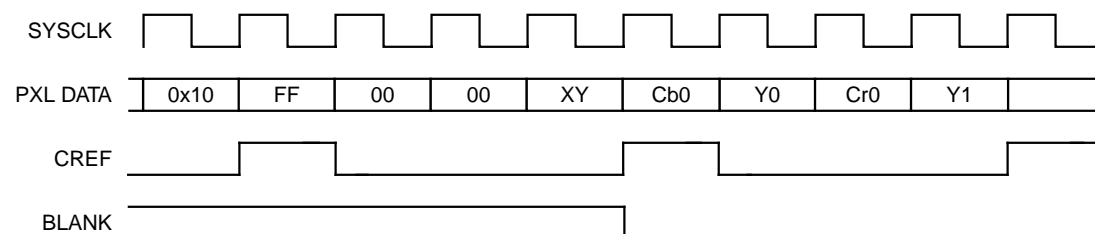
Figure 9.20 Video and Control Output Timing
