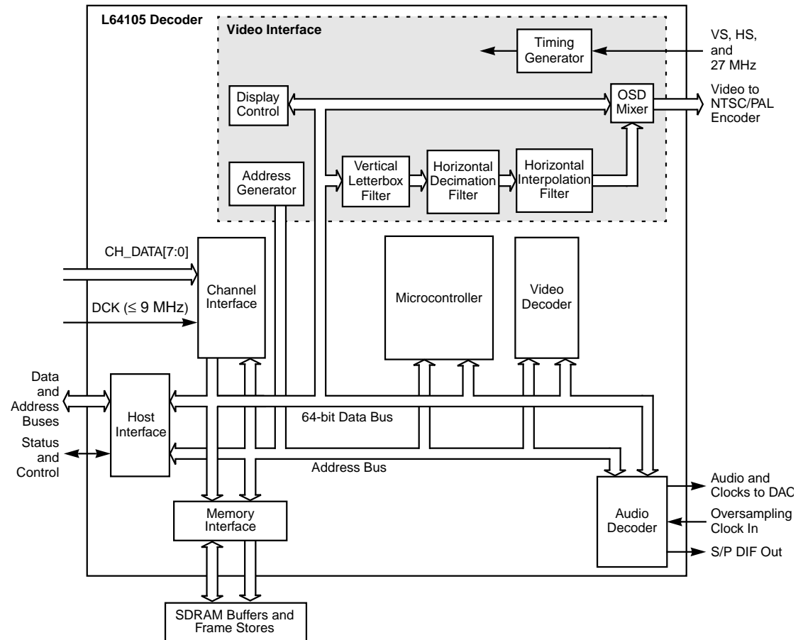
Figure 9.1 Video Interface Block Diagram
