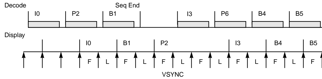
Figure 8.10 Example of Sequence End Processing
