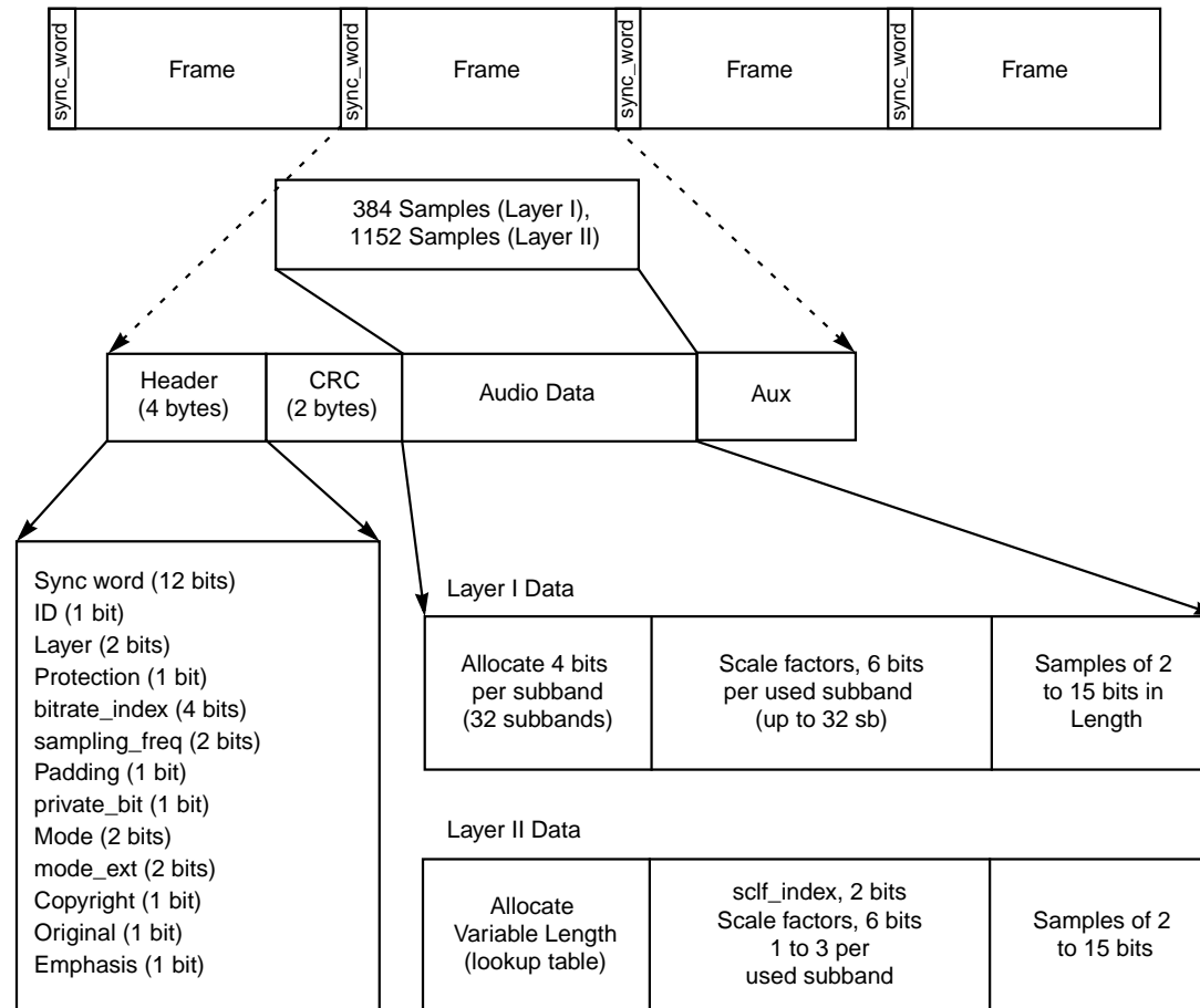
Figure 10.2 MPEG Audio Bitstream Syntax
