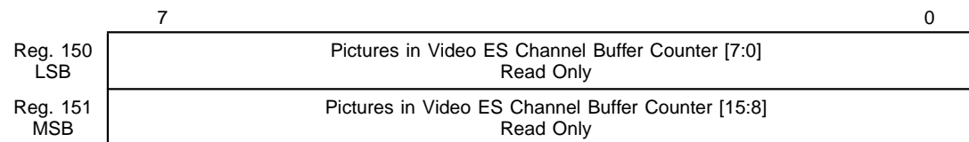
Figure 4.52 Registers 150 and 151 (0x096 and 0x097) Pictures in Video ES Channel Buffer Counter [15:0]
