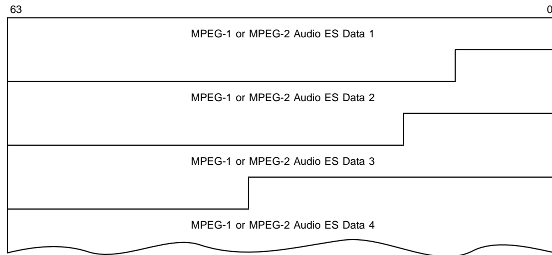
Figure 6.12 Audio ES Channel Buffer Map for MPEG Audio
