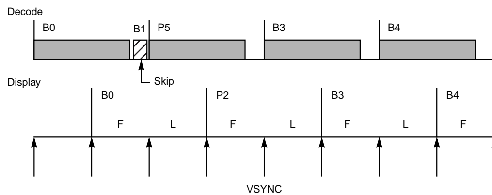
Figure 8.5 Single Skip with and without Display Freeze
