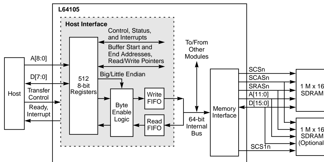
Figure 5.1 Host Interface Block Diagram
