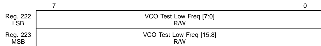
Figure 4.69 Registers 222 and 223 (0x0DE and 0x0DF) VCO Test Low Freq [15:8]
