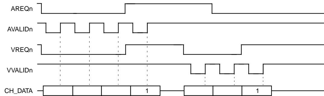
Figure 6.2 Asynchronous Channel Interface Timing
