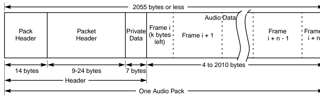
Figure 10.4 Linear PCM Packet Syntax
