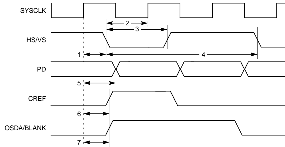
Figure 11.12 Video Interface Timing
