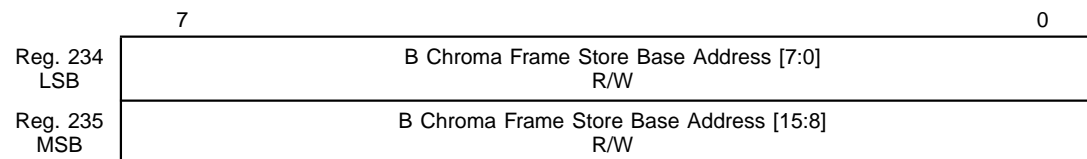
Figure 4.75 Registers 234 and 235 (0x0EA and 0x0EB) B Chroma Frame Store Base Address [15:0]
