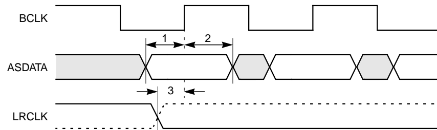
Figure 11.13 Serial PCM Data Out Timing
