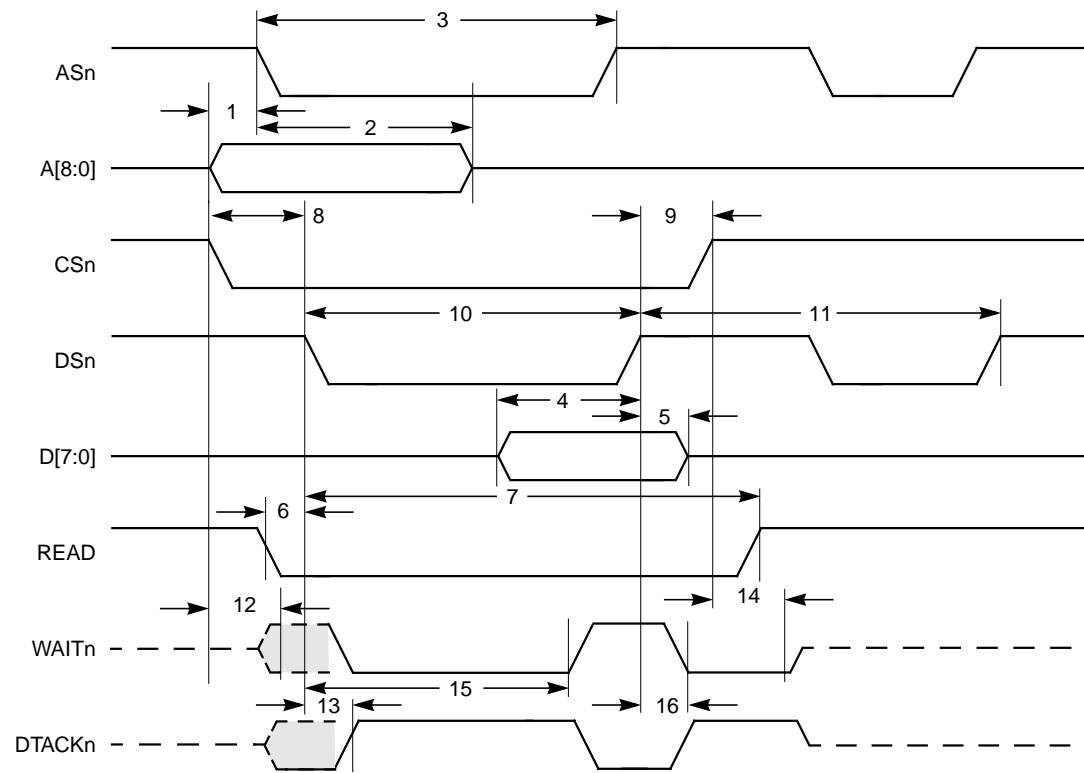
Figure 11.5 Host Write Timing (Motorola Mode)
