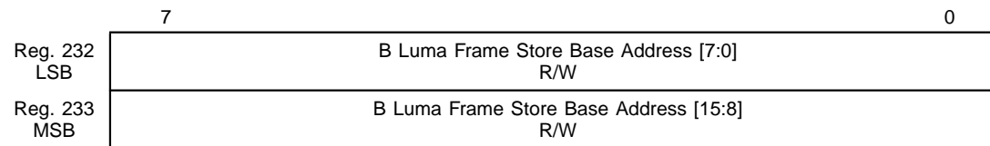
Figure 4.74 Registers 232 and 233 (0x0E8 and 0x0E9) B Luma Frame Store Base Address [15:0]
