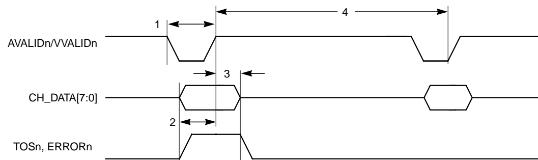
Figure 11.9 Asynchronous Channel Write Timing
