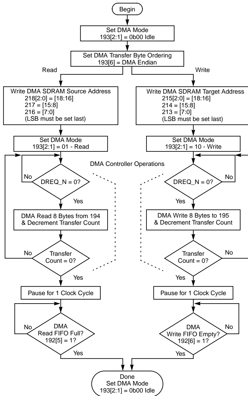
Figure 5.9 DMA SDRAM Read/Write Flowchart
