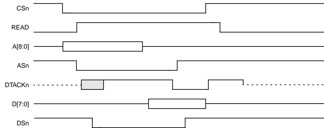
Figure 5.3 Motorola Mode Read Timing
