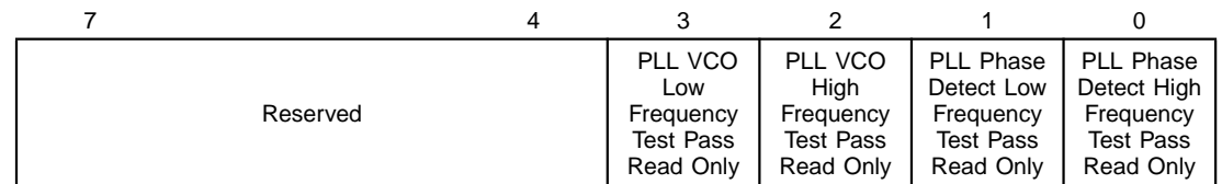
Figure 4.68 Register 221 (0x0DD)
