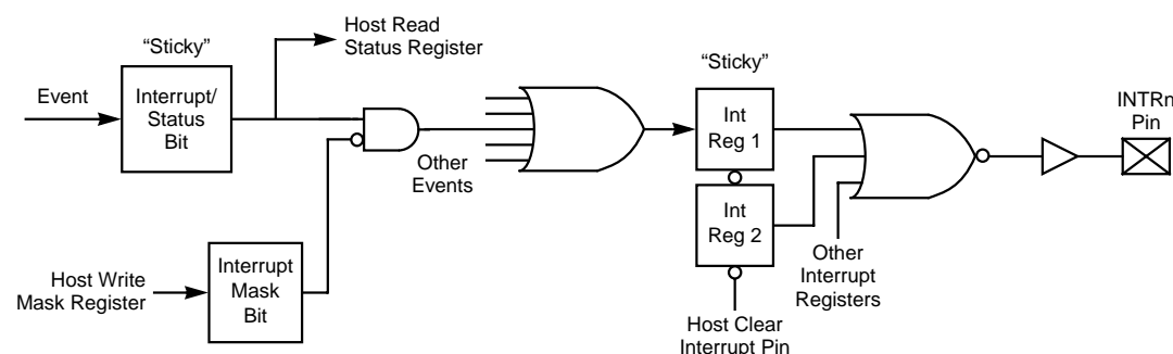
Figure 5.7 Interrupt Structure
