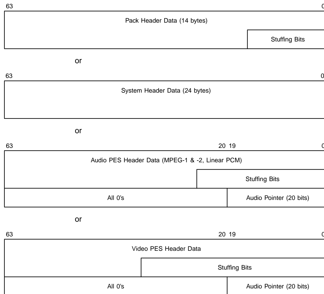
Figure 6.10 System Channel Buffer Map for Program Streams
