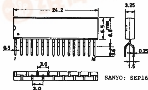
Package Dimensions (unit: mm) 3020A
