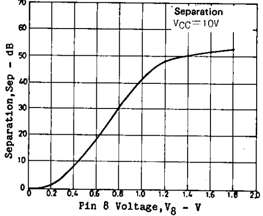
SNC Characteristic (Fig 3b)
