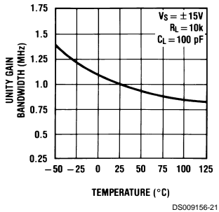
Gain Bandwidth
