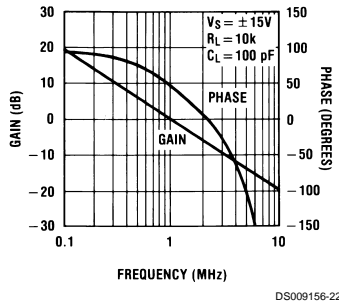
Bode Plot
