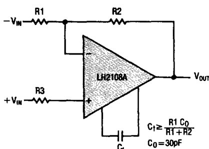
Standard Compensation Circuit
