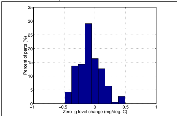
Figure 11. x-axis Zero-g level change Vs temperature
