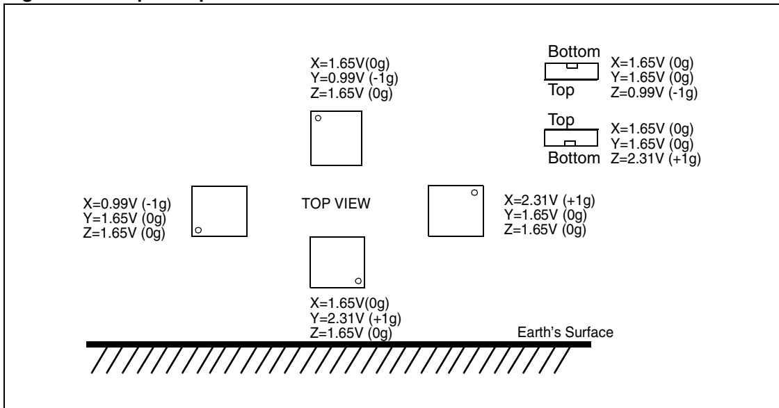
Figure 4 refers to LIS3L06AL device powered at 3.3V.
