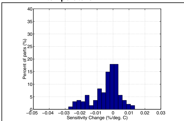
Figure 15. y-axis sensitivity change Vs temperature
