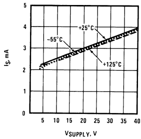
Power Drain vs V_{SUPPLY}
