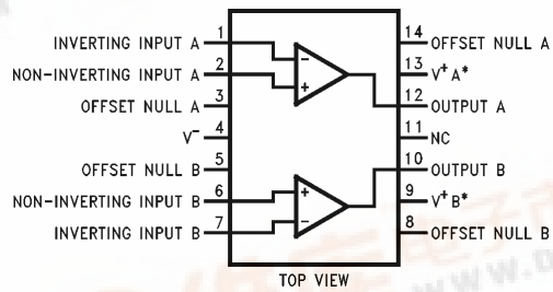
Dual-In-Line Package
