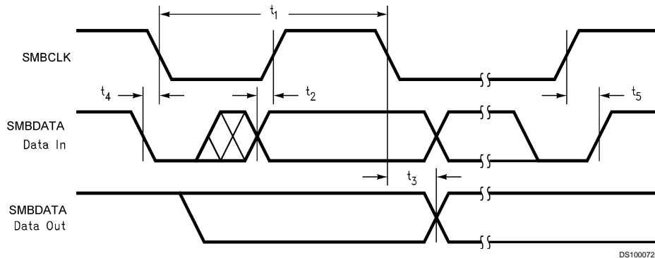
FIGURE 1. Serial Bus Timing Diagram
