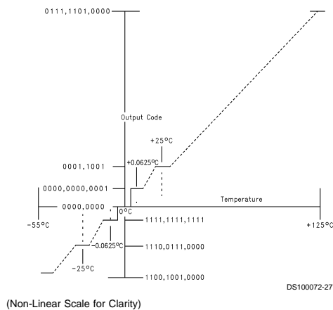
FIGURE 10. 12-bit Temperature-to-Digital Transfer Function
