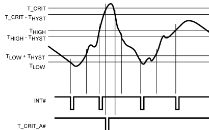
FIGURE 15. Extended One-Time Interrupt
