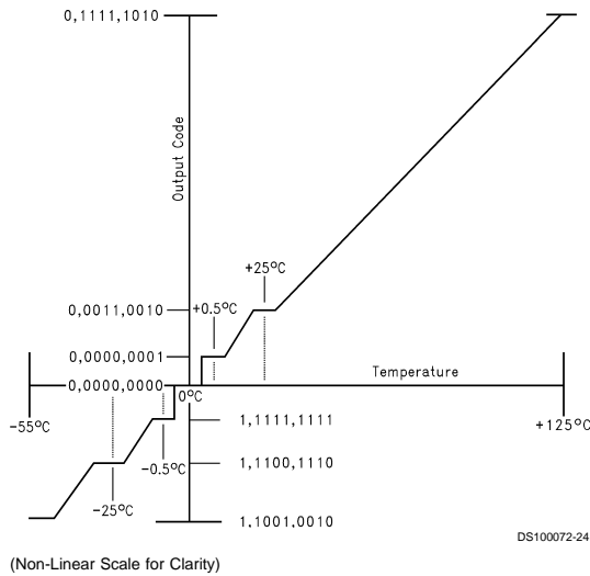
FIGURE 9. 9-bit Temperature-to-Digital Transfer Function
