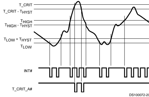
FIGURE 14. Extended Repetitive Interrupt Mode
