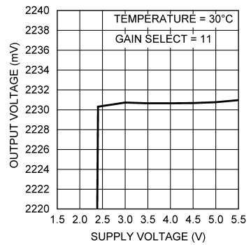
Output Voltage vs. Supply Voltage Gain Select = 11
