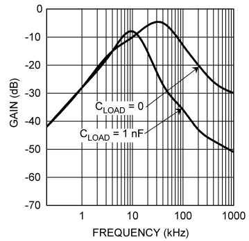
Supply-Noise Gain vs. Frequency
