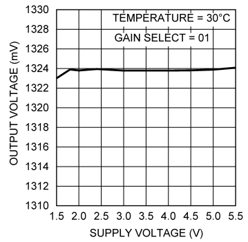
Output Voltage vs. Supply Voltage Gain Select = 01
