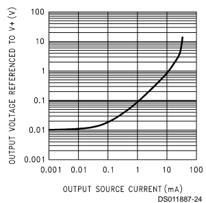
Output Characteristics vs Sourcing Current
