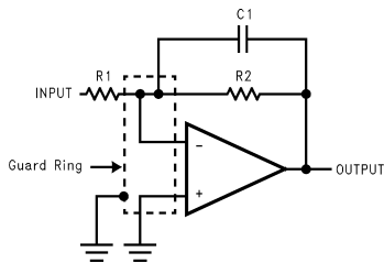
Inverting Amplifier
