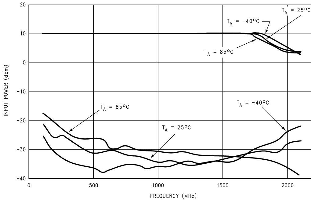
LMX2346 F IN Sensitivity vs Frequency at 3.0V
