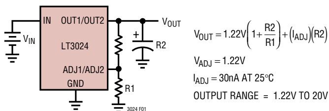
Figure 1. Adjustable Operation
