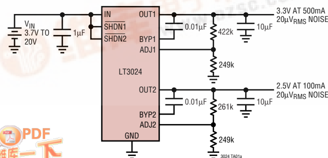
3.3V/2.5V Low Noise Regulators
