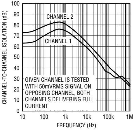
Channel-to-Channel Isolation
