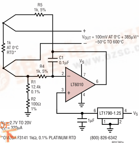
Single Supply Current Source for Platinum RTD
