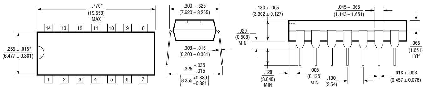
N Package 14-Lead PDIP (Narrow 0.300) (LTC DWG # 05-08-1510)
