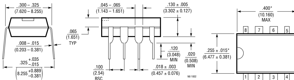
N Package 8-Lead PDIP (Narrow 0.300) (LTC DWG # 05-08-1510)
