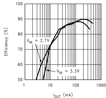
Efficiency vs. Load Current ( V_{OUT} = 8V , f_S = 1.3\text{ MHz} )
