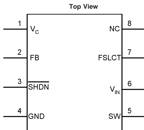
8-Lead Plastic MSOP NS Package Number MUA08A
