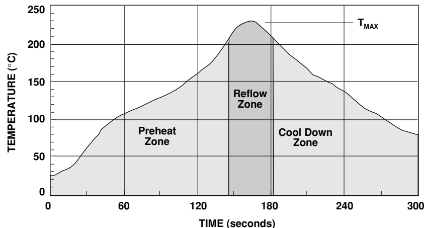
Figure 17. Surface Mount Assembly Profile.
