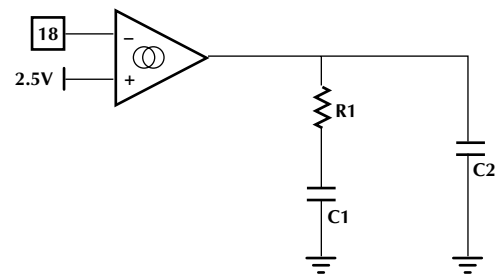
Figure 2. Compensation Network
