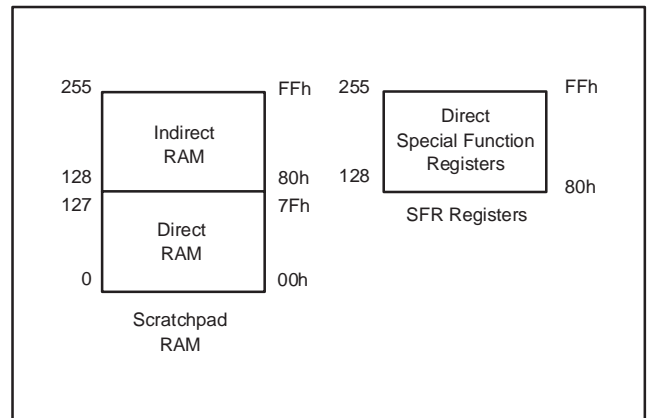
Figure 22. Register Map
