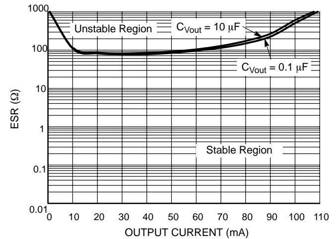
Figure 9. Output Stability with Output Capacitor Change
