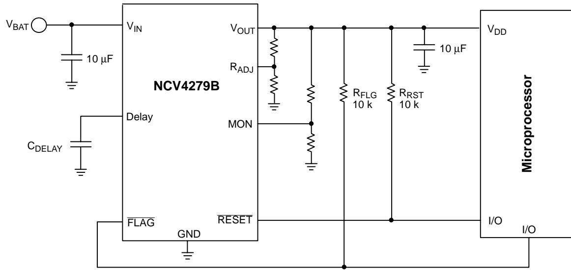
Figure 1. Application Diagram
