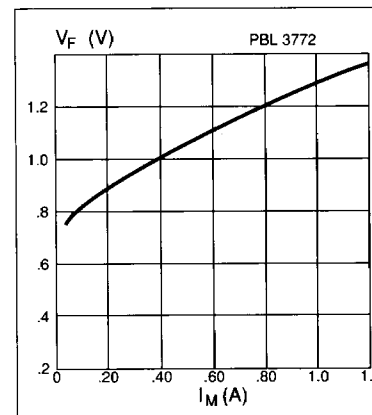
Figure 12. Typical lower diode voltage vs. output current.
