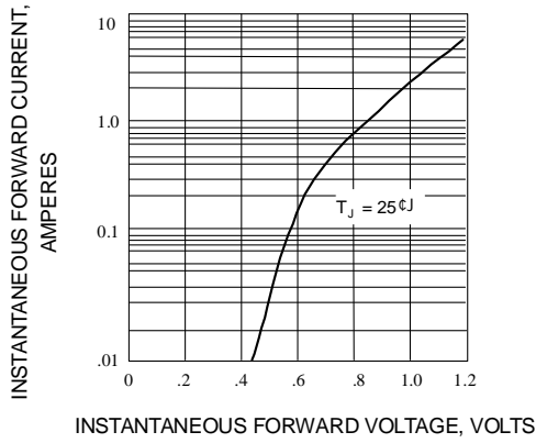
Fig. 1-TYPICAL FORWARD CHARACTERISTICS
