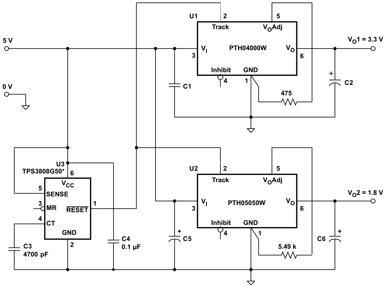
Figure 14. Auto-Track Circuit
