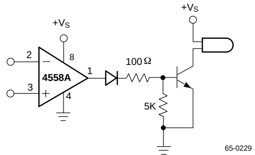
Figure 19. Lamp Driver
