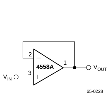
Figure 18. Voltage Follower
