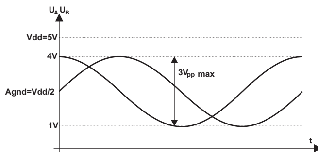
Input signals requirements
