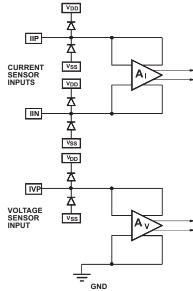
Figure 4: Analog input internal configuration
