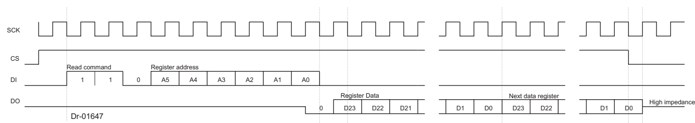
Figure 8: SPI waveforms
