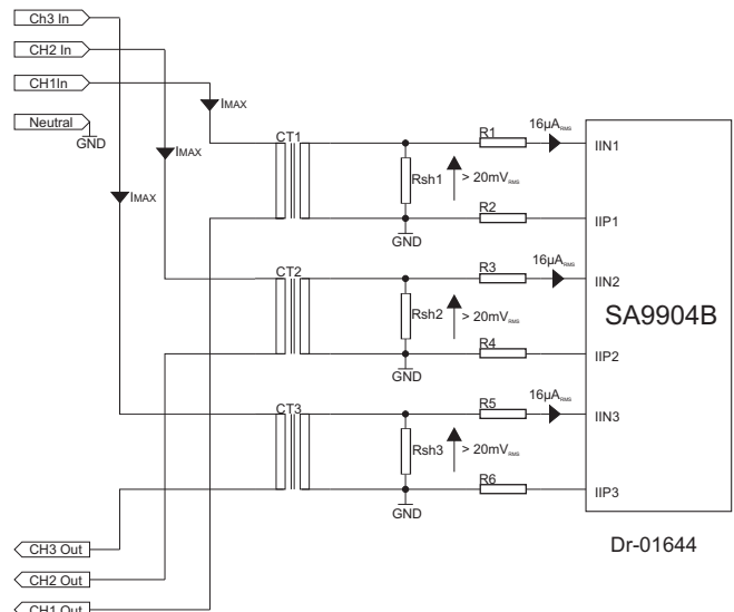
Figure 5: Current sense input configuration
