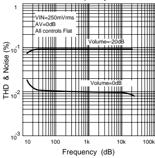
Fig.7 Distortion & Noise vs. Frequency
