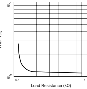
Fig.8 Distortion vs. Load Resistance
