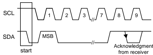
Fig. 19 Acknowledge on the I 2 C BUS
