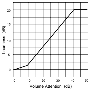
Fig.1 Loudness vs. Volume Attention
