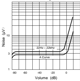
Fig.4 Noise vs. Volume/Gain settings
