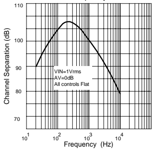
Fig.9 Channel Separation(L→R) vs. Frequency
