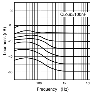
Fig.2 Loudness vs. Frequency vs. volume Attenuation
