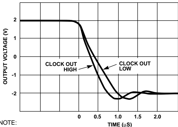
FIGURE 19. VOLTAGE FOLLOWER LARGE SIGNAL PULSE RESPONSE (NOTE)
