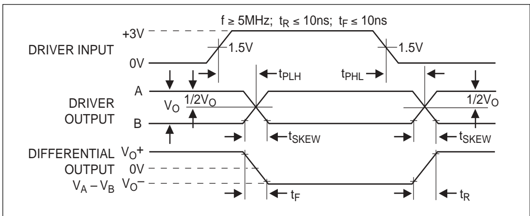
Figure 36. Driver Propagation Delays
