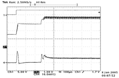
Startup 700mA Flash, V_{in} = 3.6V , V_{out} = 3.65V
