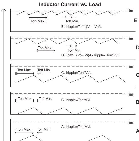
Figure 1. Inductor Current vs. Load
