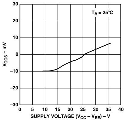
TPC 15. V_{00S} vs. Supply Voltage
