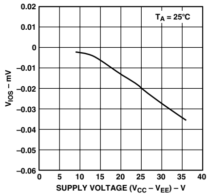
TPC 13. V_{10S} vs. Supply Voltage
