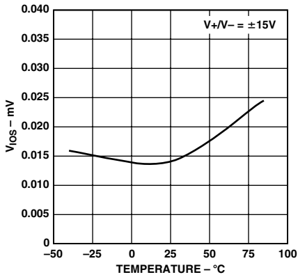
TPC 12. V_{10S} vs. Temperature
