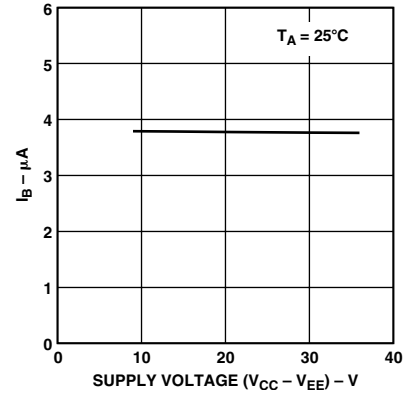
TPC 17. I_B vs. Supply Voltage
