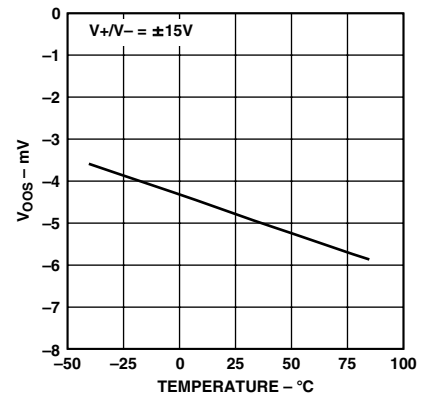
TPC 14. V_{00S} vs. Temperature
