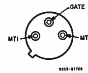
Modified TO-205
