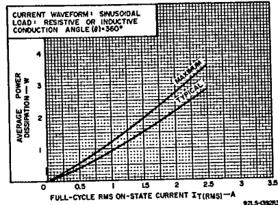
Fig. 2—Power dissipation vs. on-state current.
