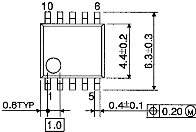
OUTLINE DRAWING SSOP10-P-225-1.00
