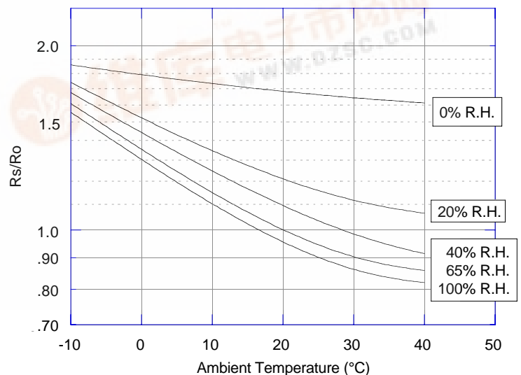
Temperature/Humidity Dependency:
