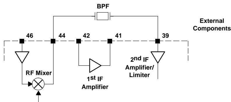
Figure 7. Bypassing the 1 st IF Amplifier
