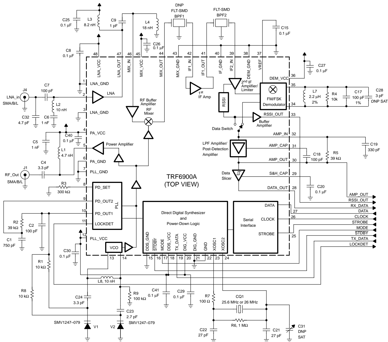
Figure 28. Typical Application Schematic for 902 to 928 MHz North American ISM Band
