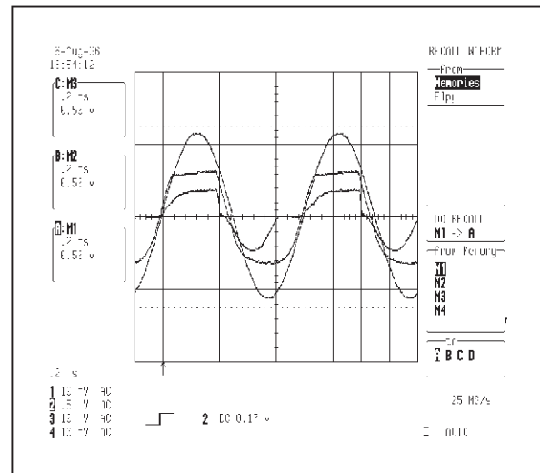
Figure 4 : Maximum Voltage Swing at Headphone Outputs ( R_L = 32\Omega )
