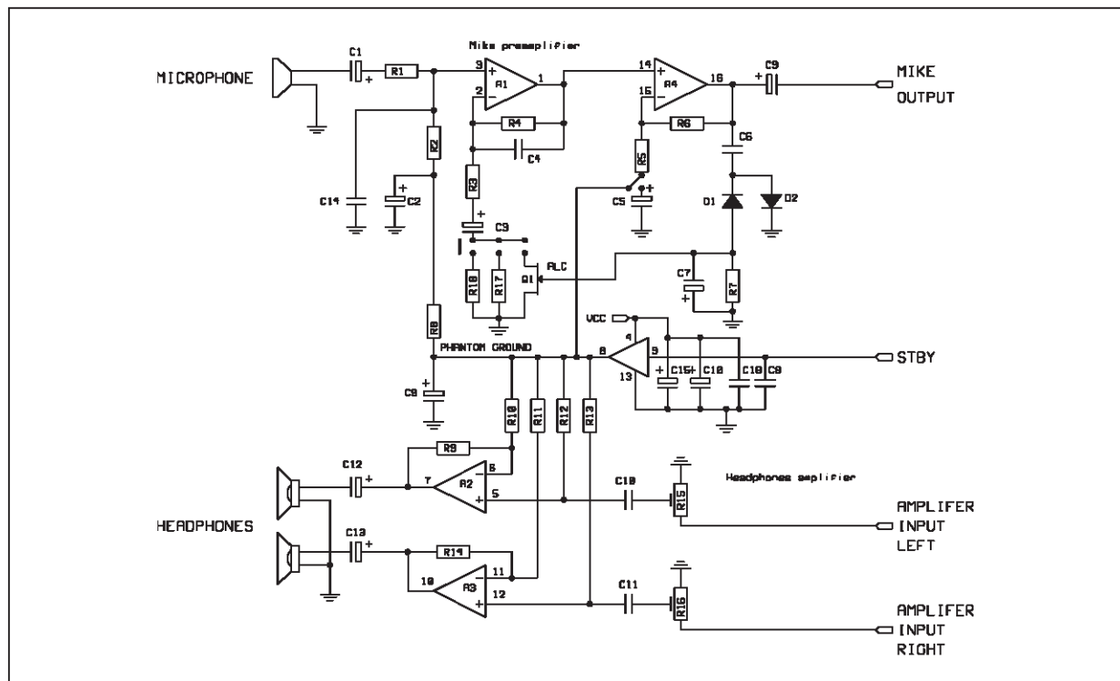
Figure 1 : Electrical Schematic
