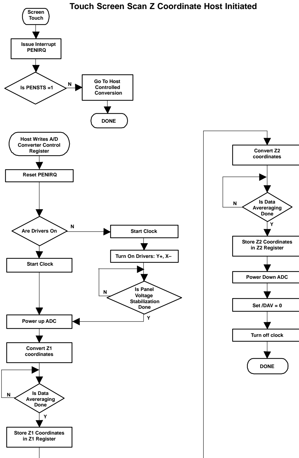
Figure 57. Z Coordinate Reading Initiated by Host.
