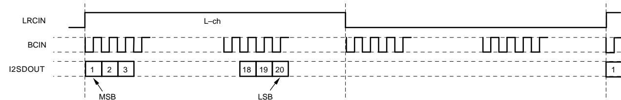
Figure 74. Audio Data Input/Output Format
