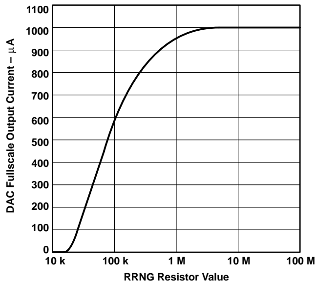
Figure 71. DAC Output Current Range vs RRNG Resistor Value.
