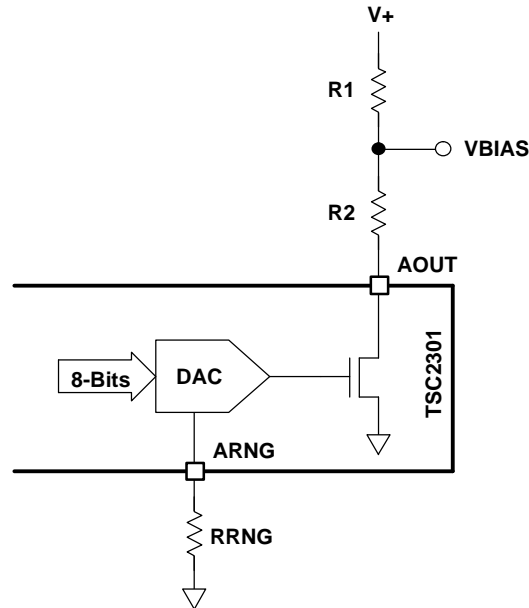
Figure 70. D/A Converter Configuration
