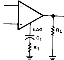
LAG COMPENSATION CIRCUIT FOR FIGURES 3, 4, AND 5
