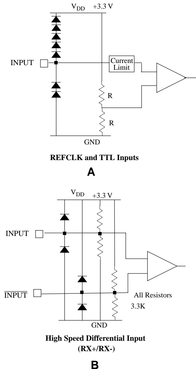
Figure 2: Input Structures
