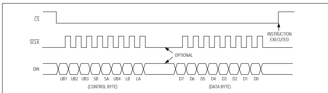
Figure 2. MAX522 3-Wire Serial-Interface Timing Diagram
