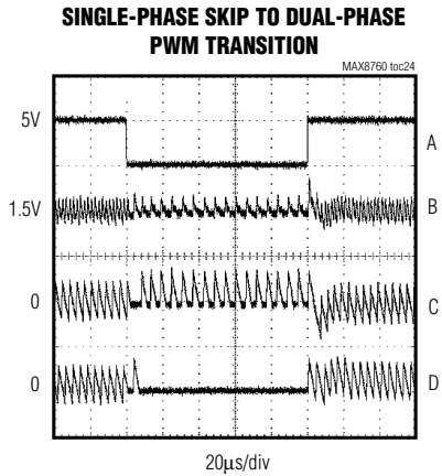
A. \overline{SKIP} = V_{CC} TO GND, 5V/div B. 1.5V OUTPUT, 50mV/div C. I_{L1} , 10A/div D. I_{L2} , 10A/div 2A LOAD
