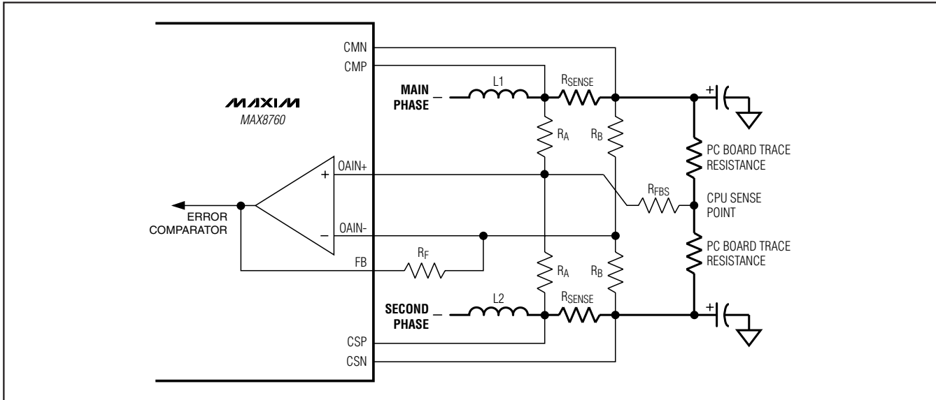
Figure 10. Voltage-Positioning Gain
