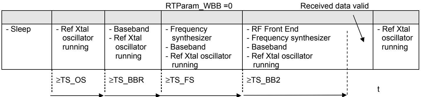
Figure 7 Standard “boosted” power up sequence from Stand By to Receiver Mode
